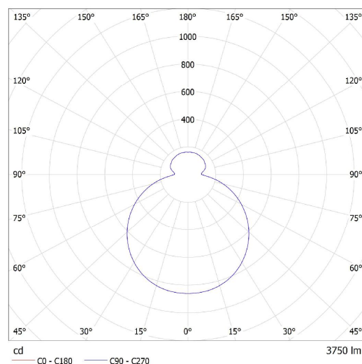
Lucis ZL3.K12.Z500 ZERO LED / LDC (Polar)
